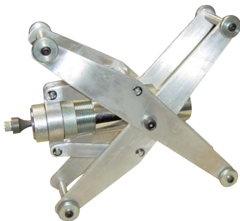
ConeBlast 1/2" Assembly Shown Fitted in Optional Centring Carriage
